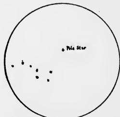
The Great Bear = Dipper pointing directly to The Star, + The 2nd Star from left in handle of Dipper is the Squaw, & next to the little Papoose
